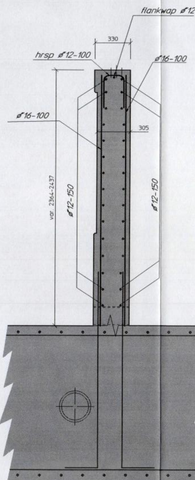
Detail 6
